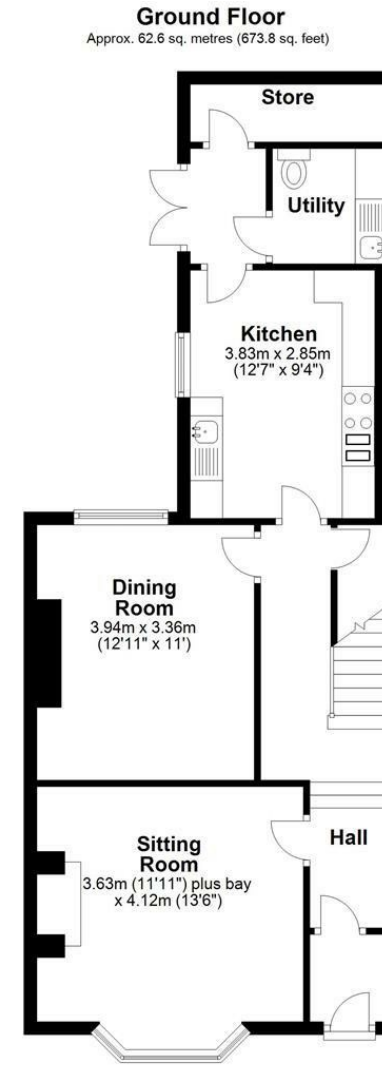
Total area: approx. 121.9 sq. metres (1312.6 sq. feet) 49 Newbiggin, Malton
